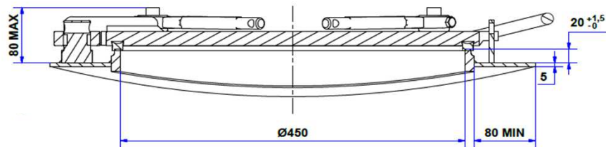
Folding Handnut
