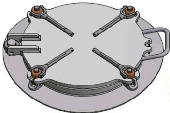
Folding Handnut
