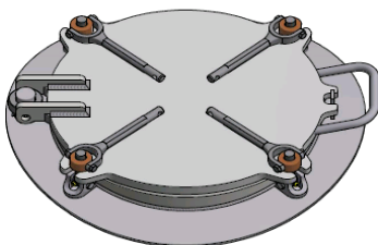
Folding Handnut
