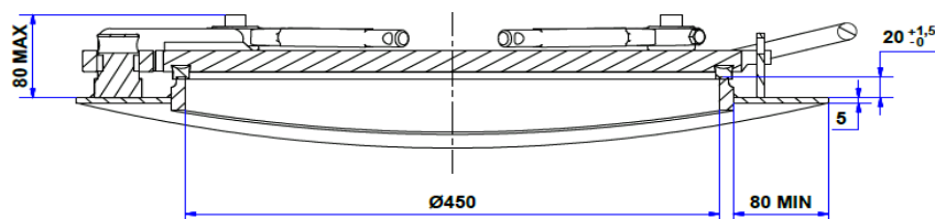
Folding Handnut
